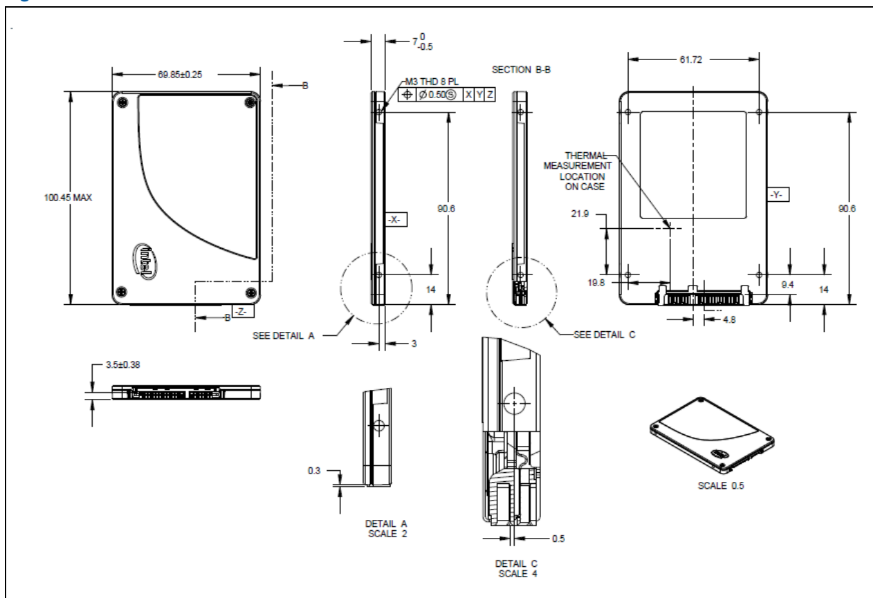
Figure 3-1: Dimensions for Full Size 2.5 inch Drives
